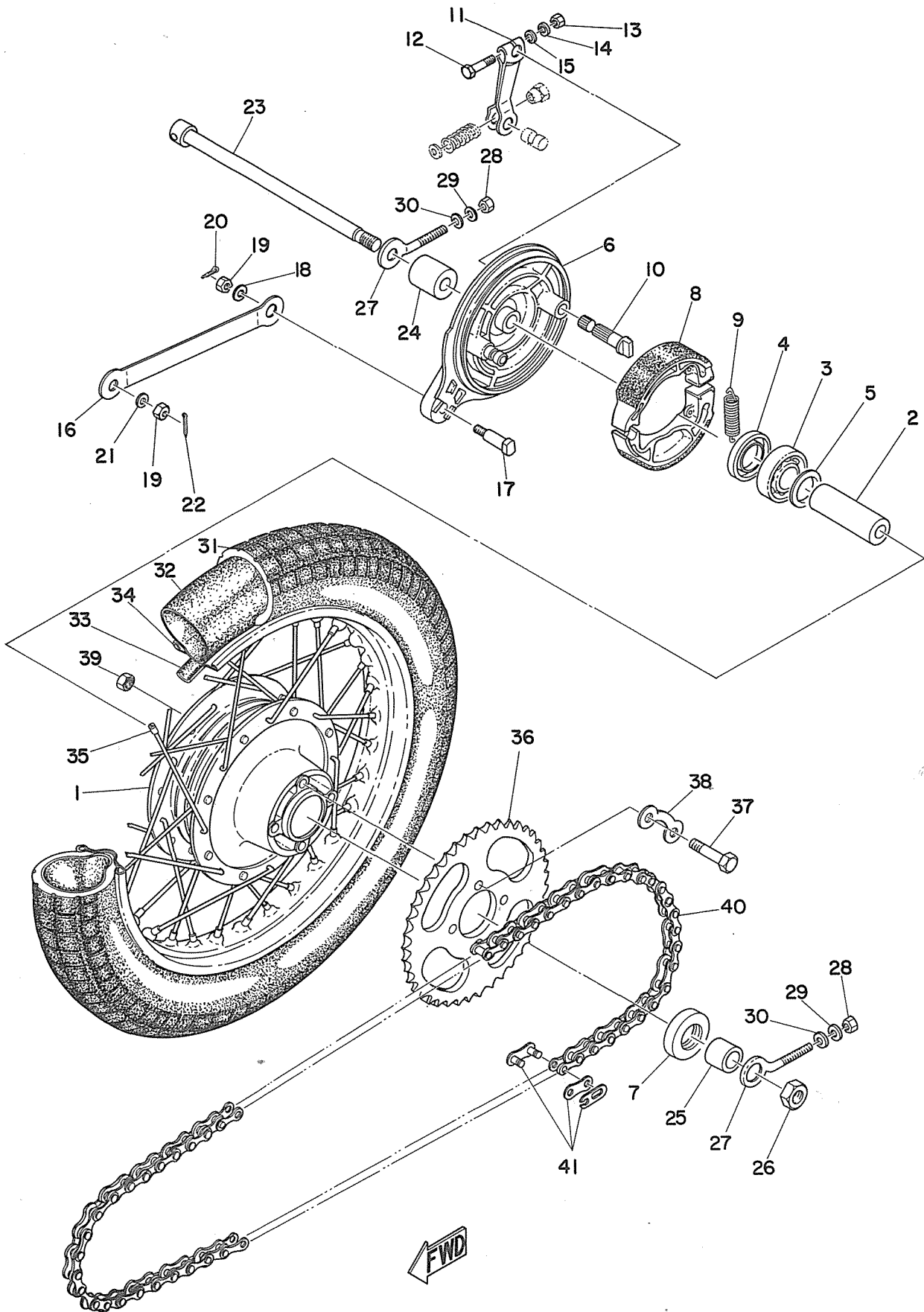
Fig. 24 REAR WHEEL
