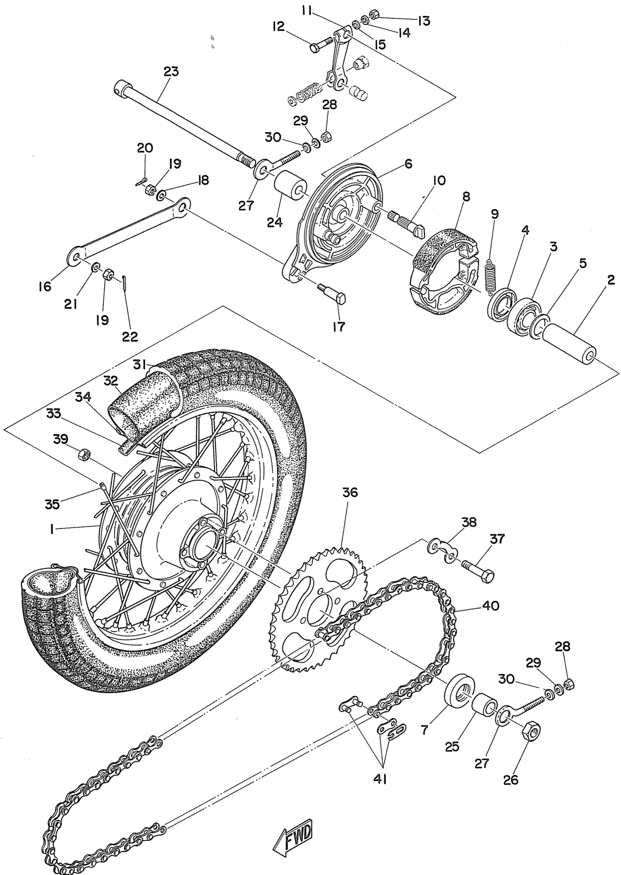
Fig. 24 REAR WHEEL
