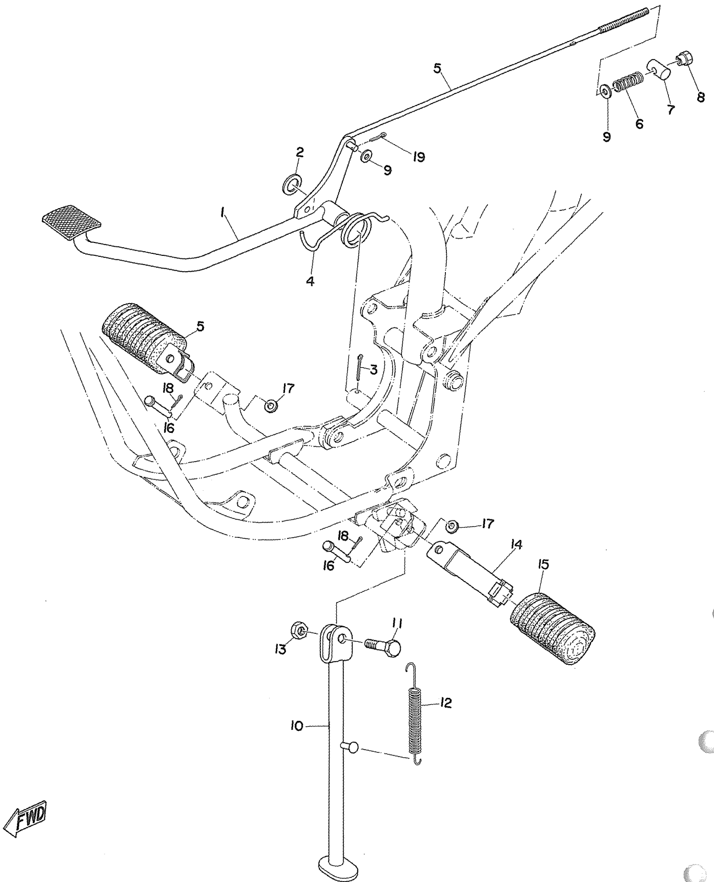
Fig. 16 STAND & BRAKE PEDAL
