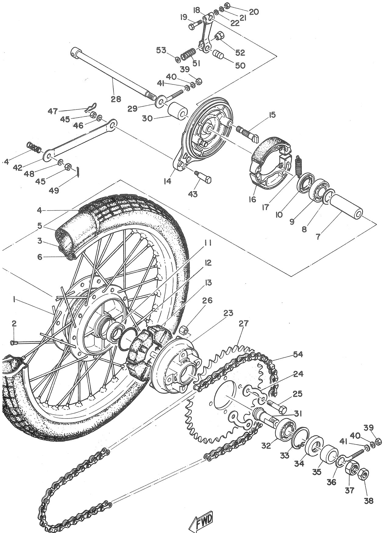
Fig. 24 REAR WHEEL
