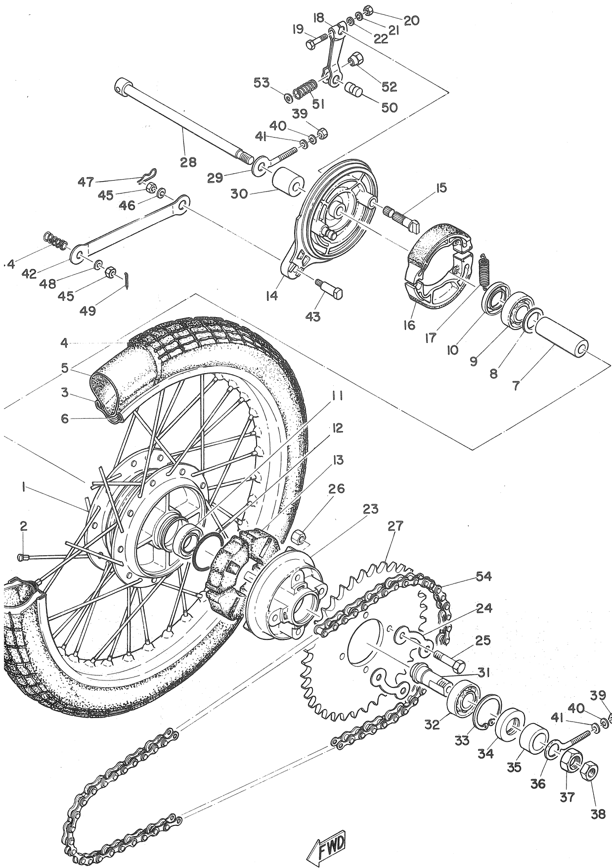
Fig. 24 REAR WHEEL
