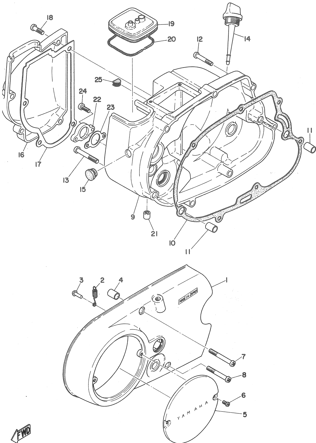
Fig. 2 CRANKCASE COVER
