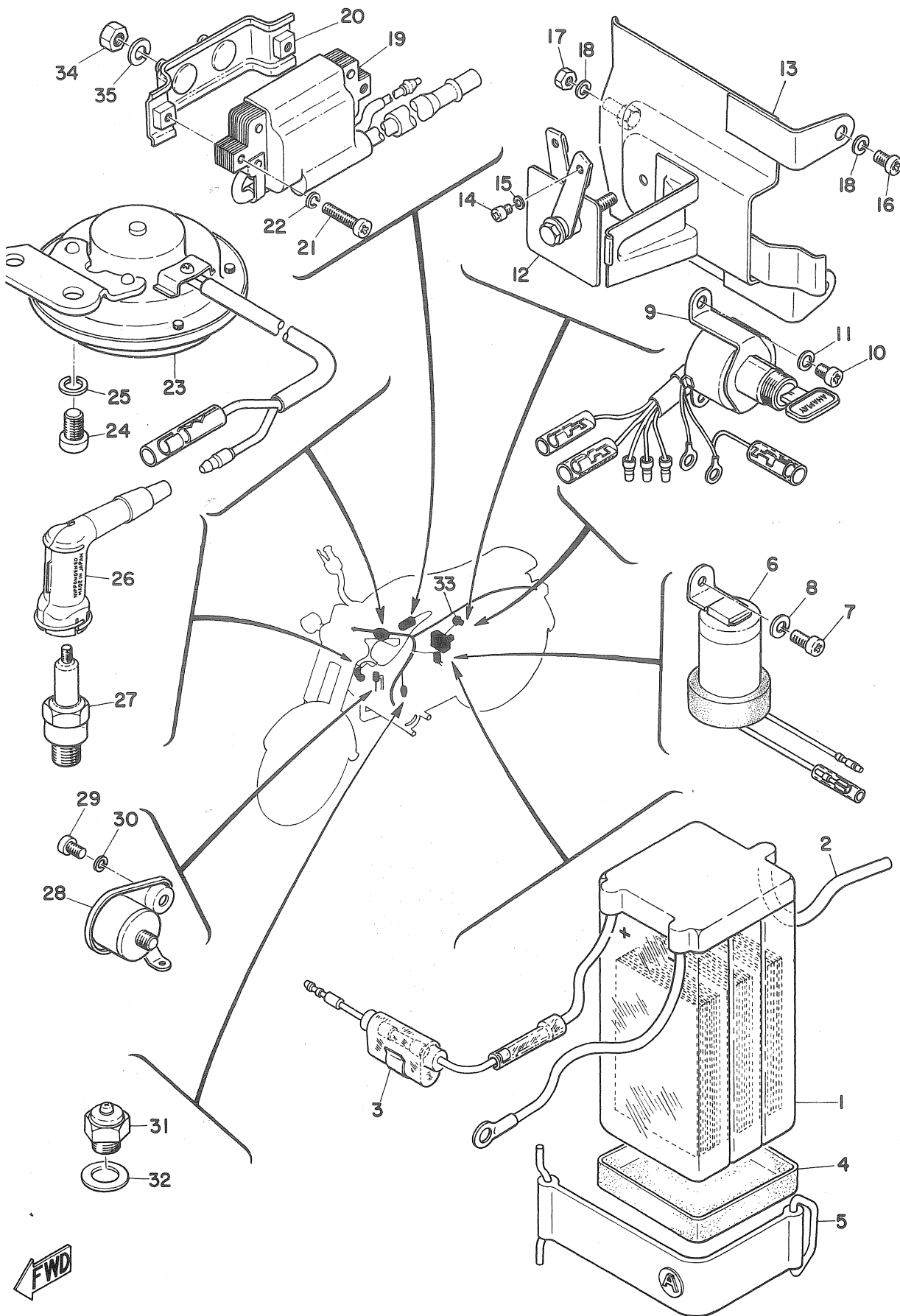
Fig. 27 ELECTRICAL
