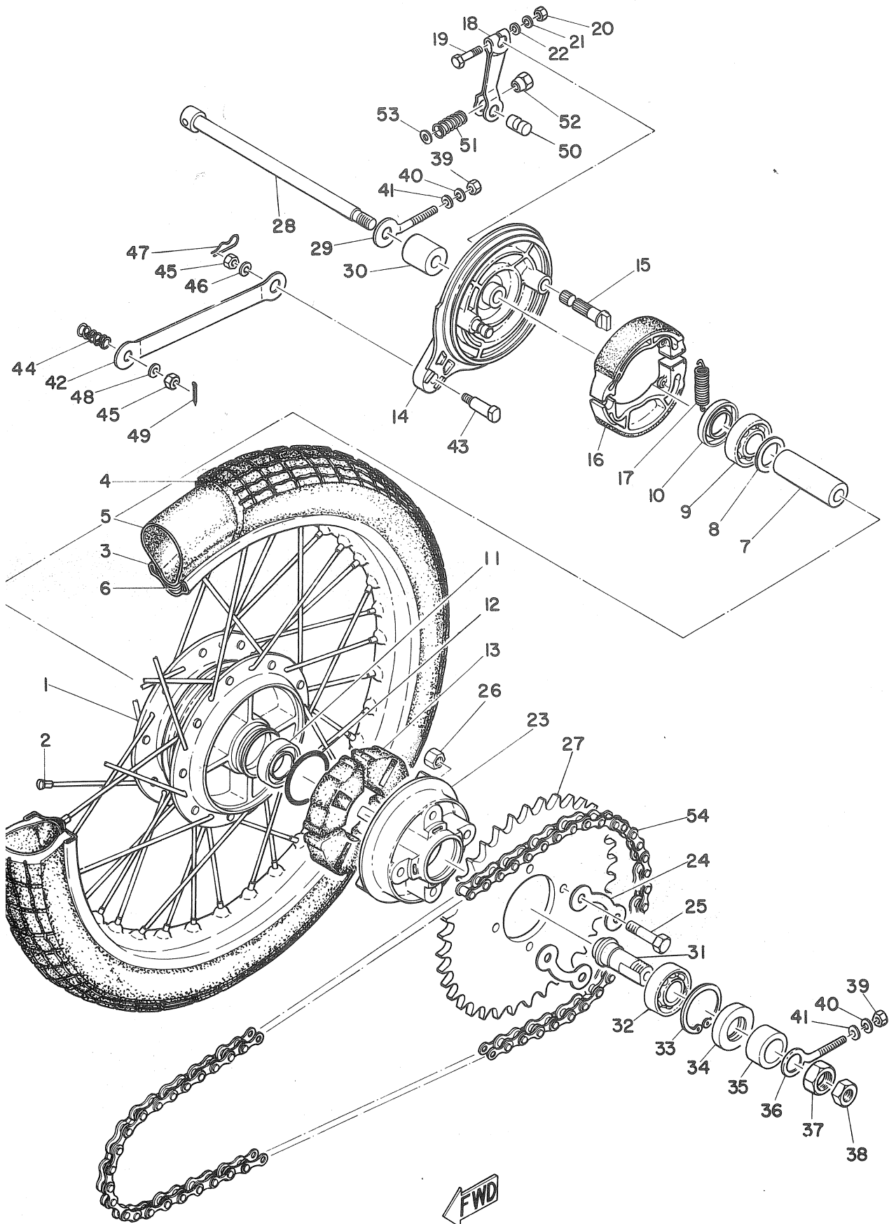
Fig. 24 REAR WHEEL
