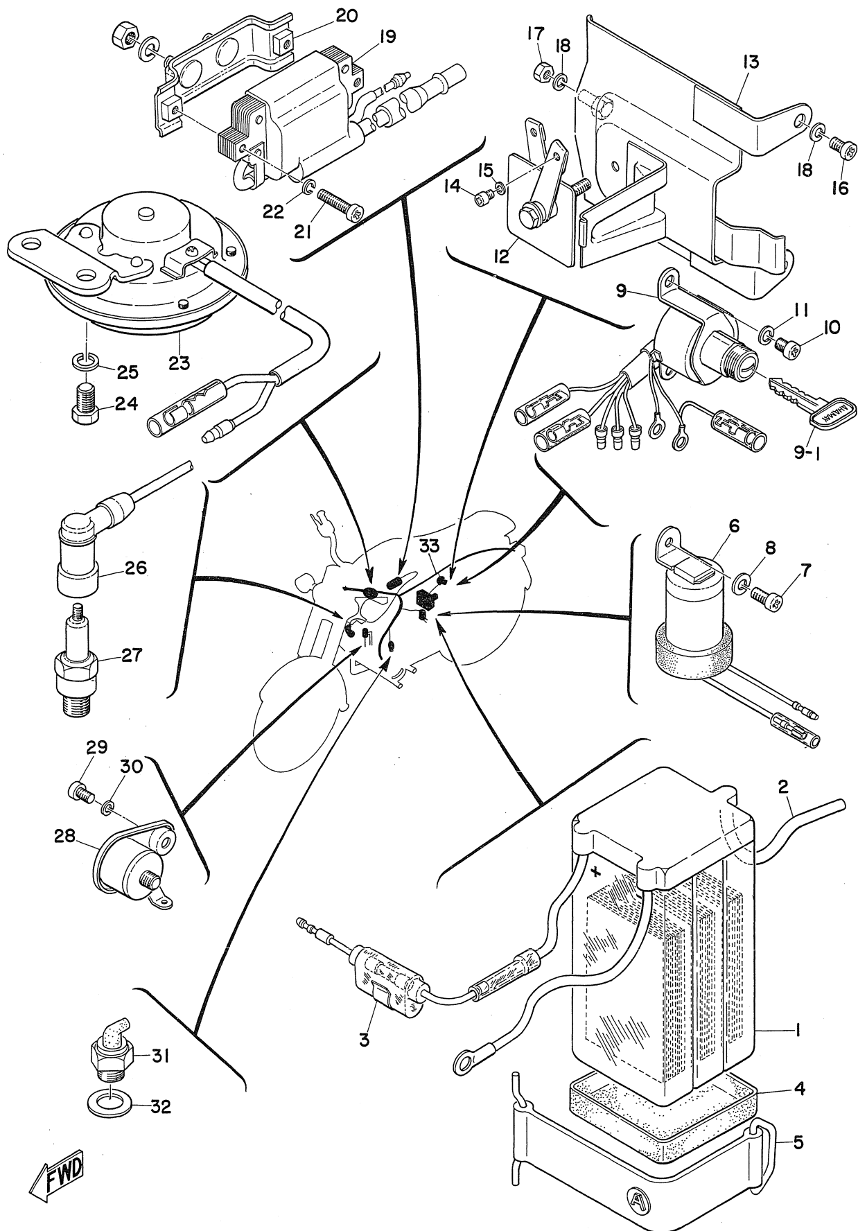
Fig. 28 ELECTRICAL
