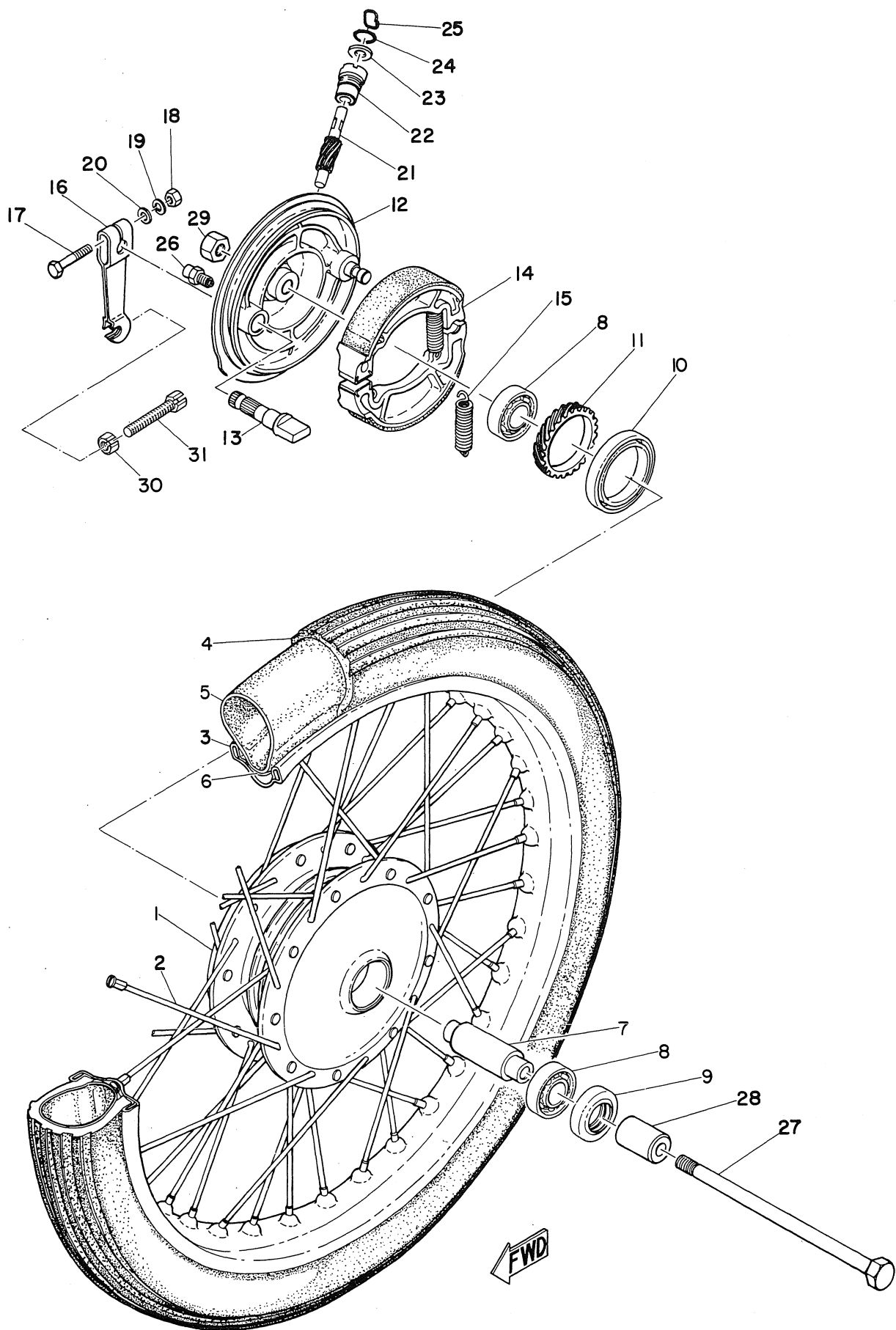
Fig. 23 FRONT WHEEL
