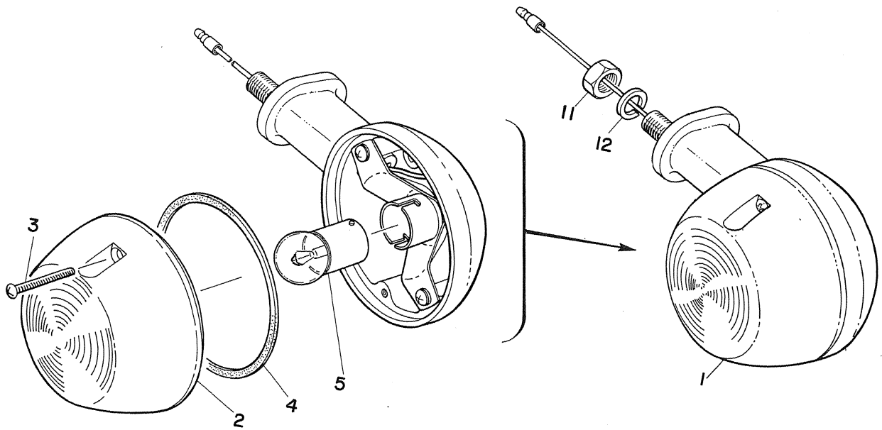
Fig. 27 FLASHER LAMP
