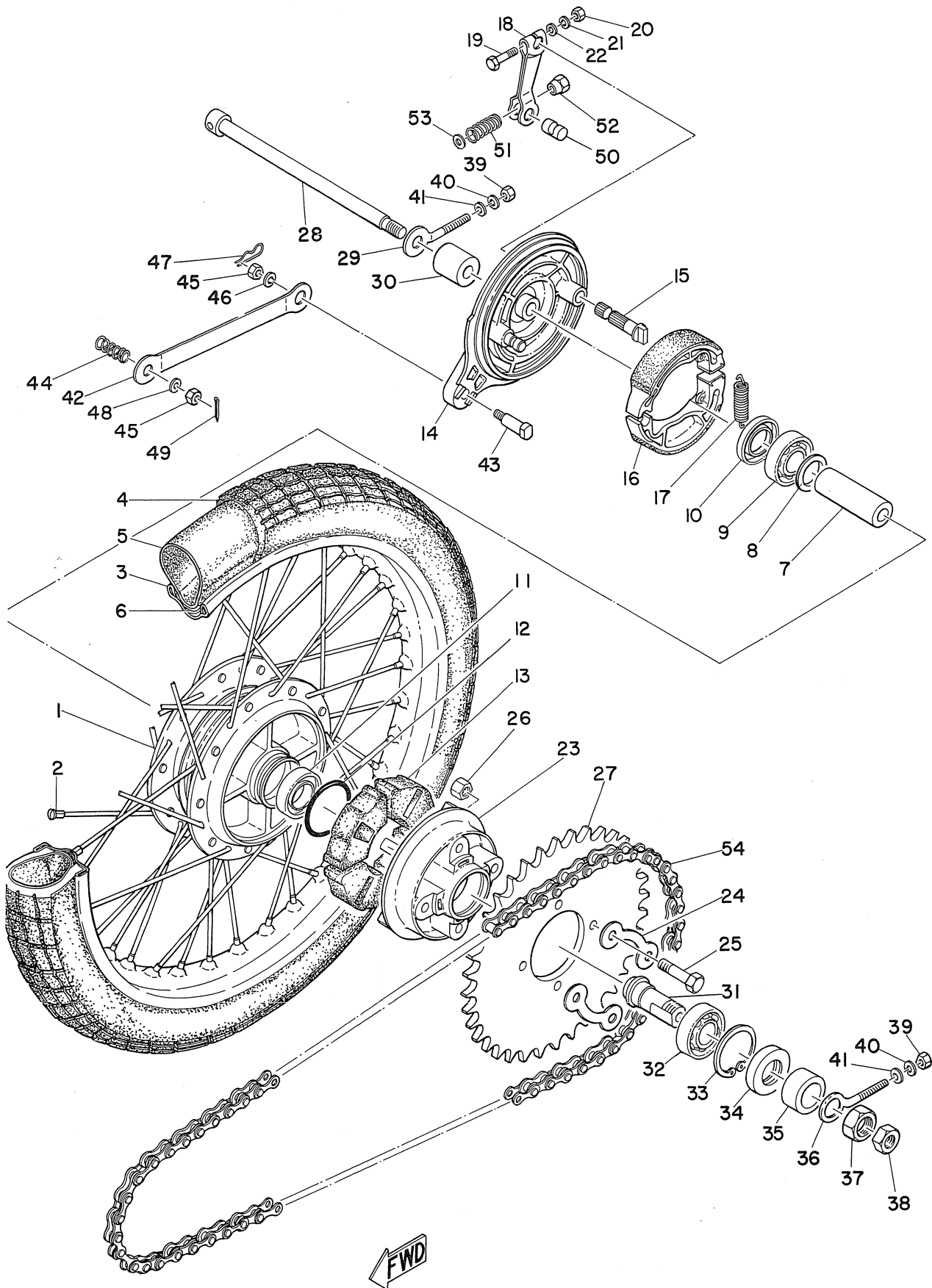
Fig. 24 REAR WHEEL
