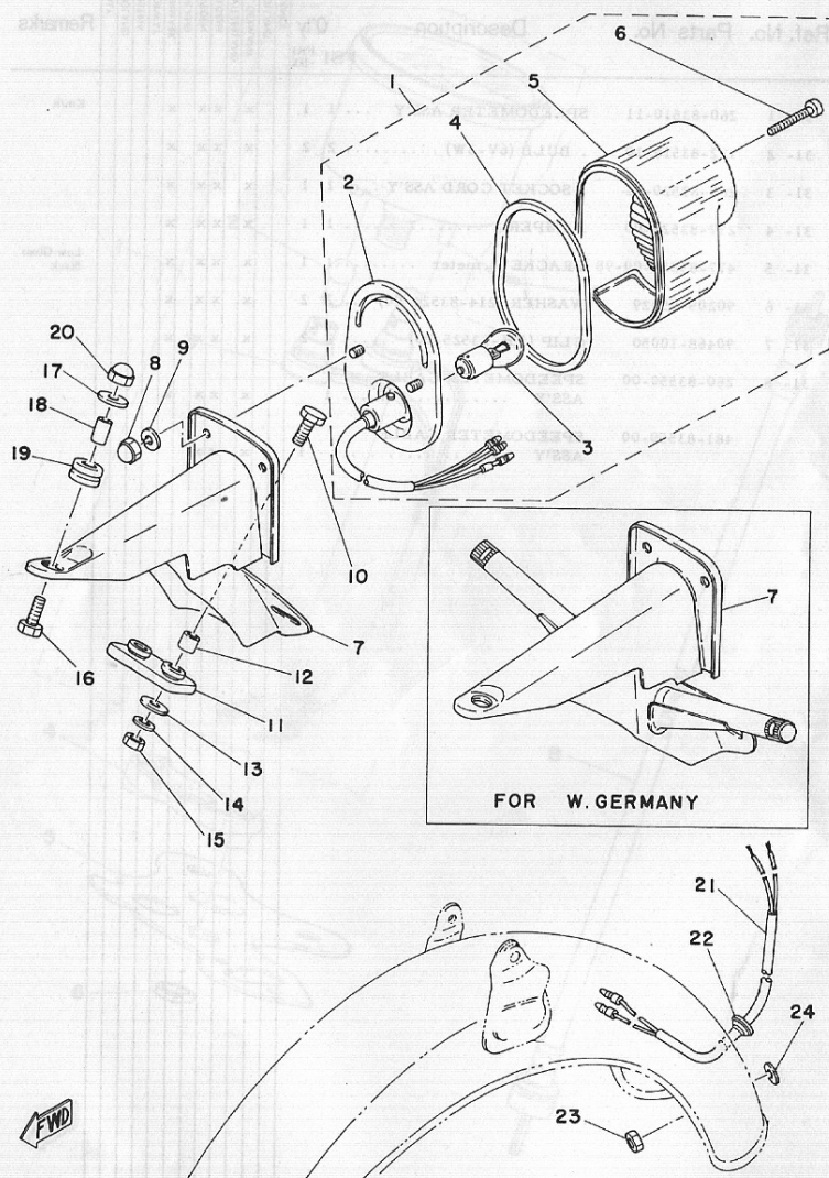
Fig. 32 TAIL LAMP
