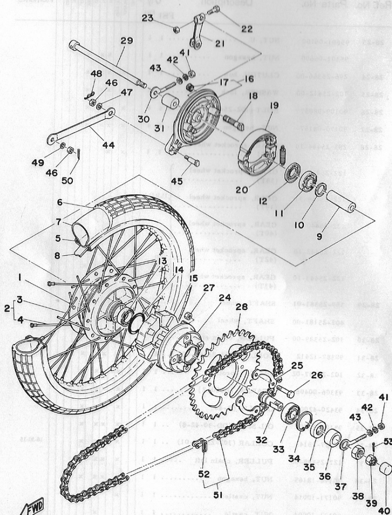
Fig. 28 REAR WHEEL
