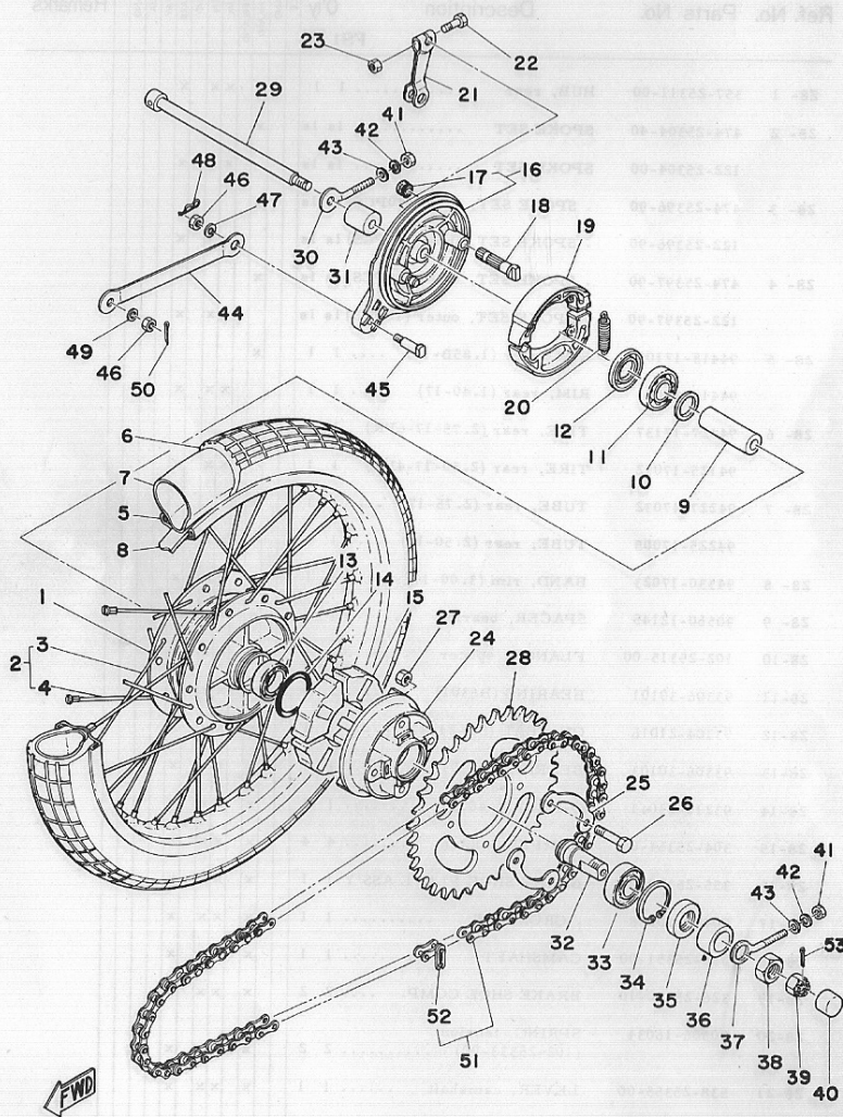
Fig. 28 REAR WHEEL
