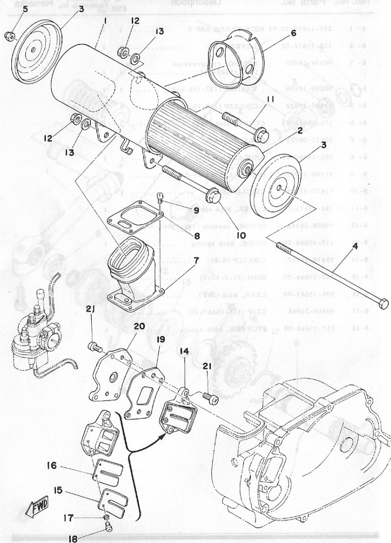
Fig. 9 INTAKE
