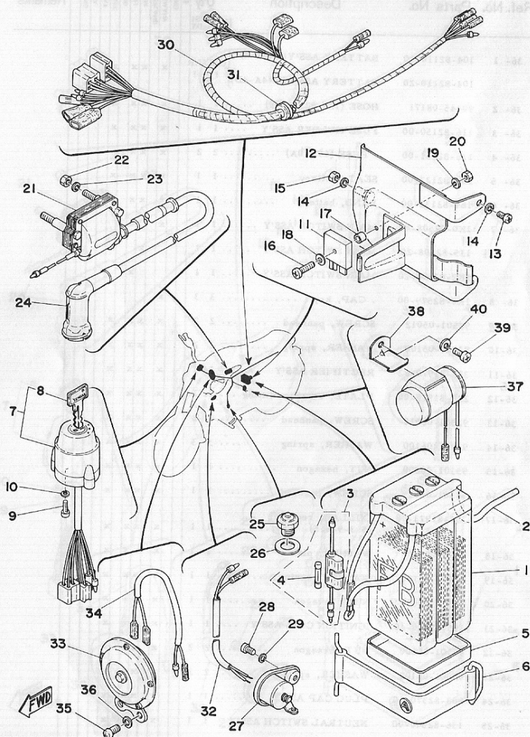
Fig. 36 ELECTRICAL
