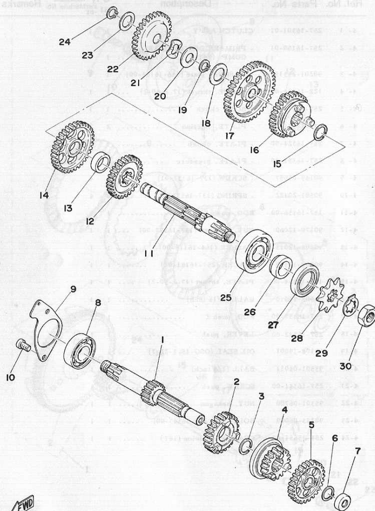
Fig. 5 TRANSMISSION
