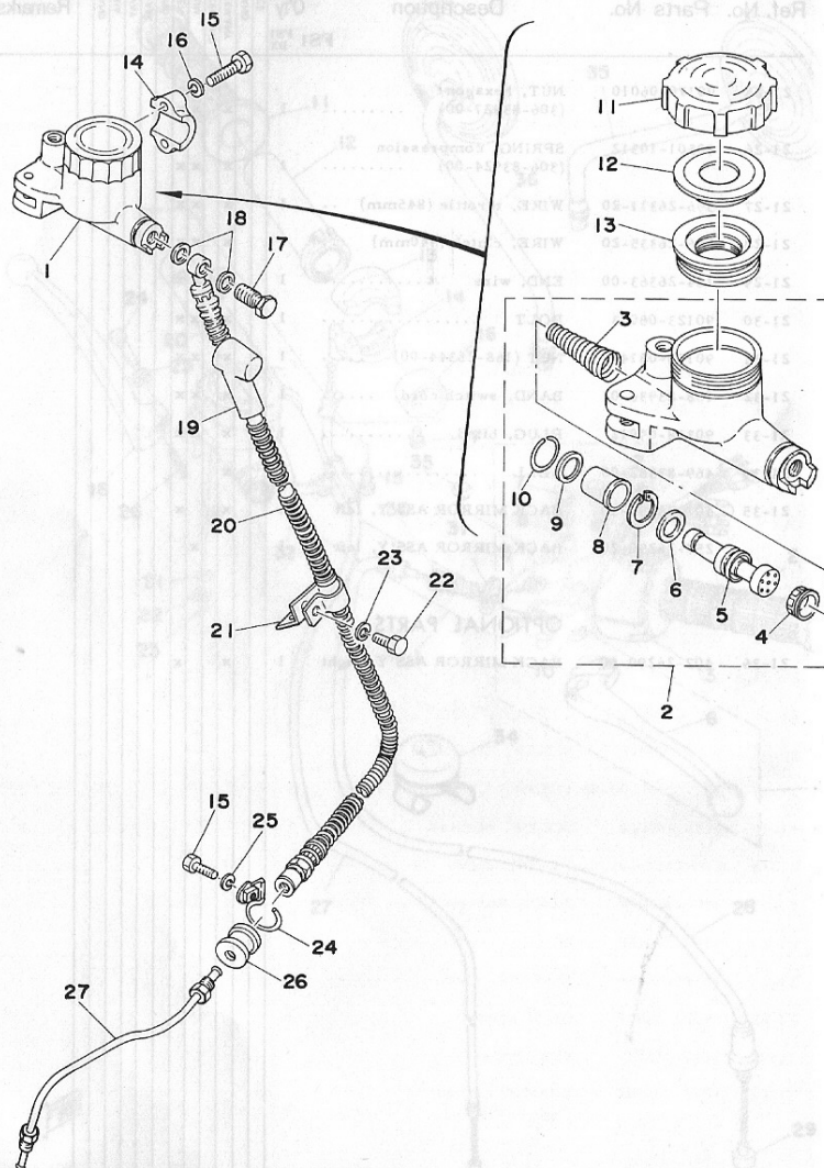
Fig. 22 MASTER CYLINDER · BRAKE HOSE
