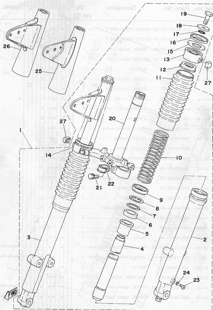
Fig. 18 FRONT FORK
