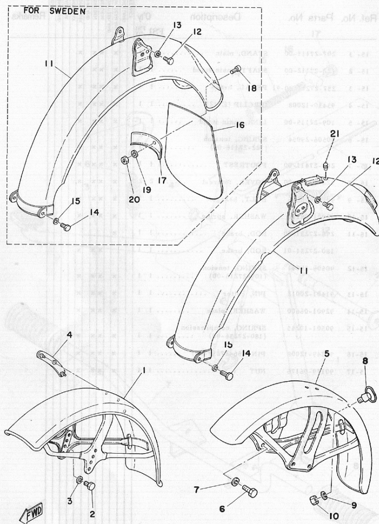
Fig. 16 FRONT FENDER · REAR FENDER
