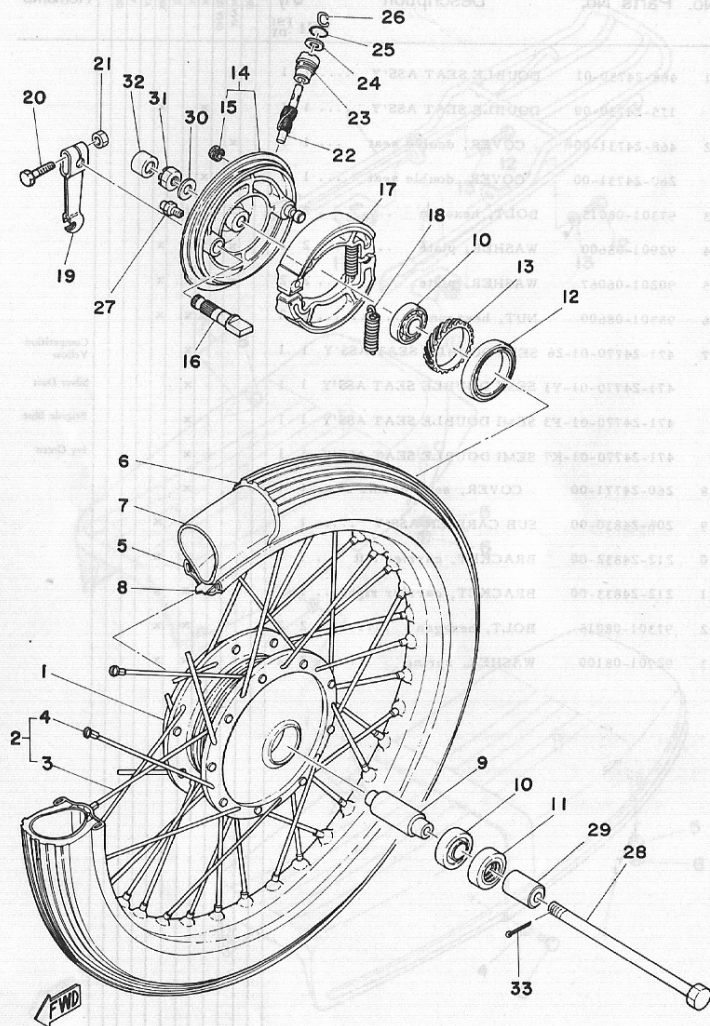
Fig. 25 FRONT WHEEL
