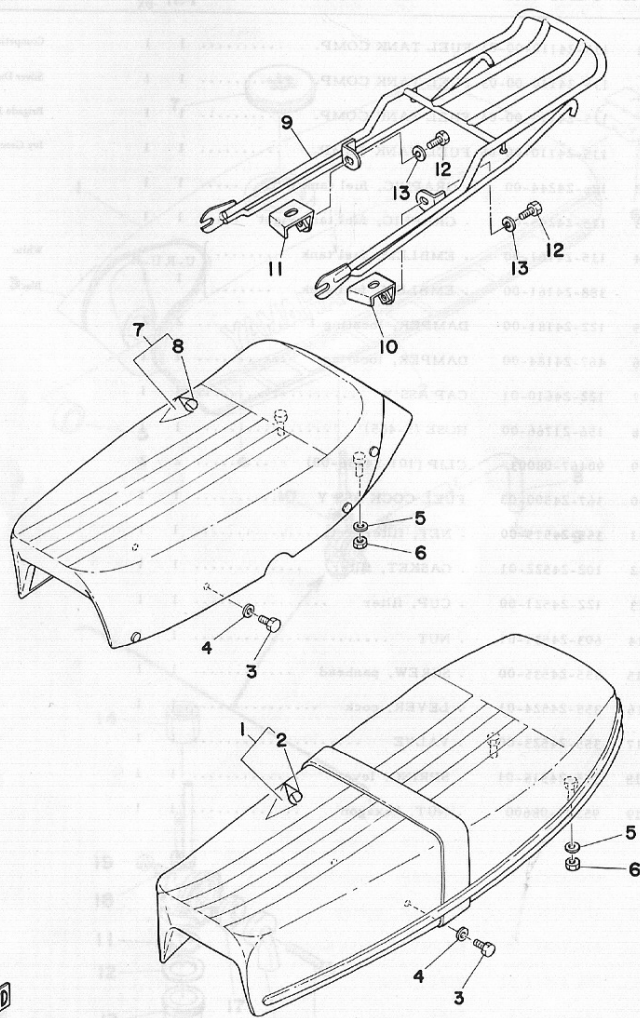
Fig. 24 SEAT
