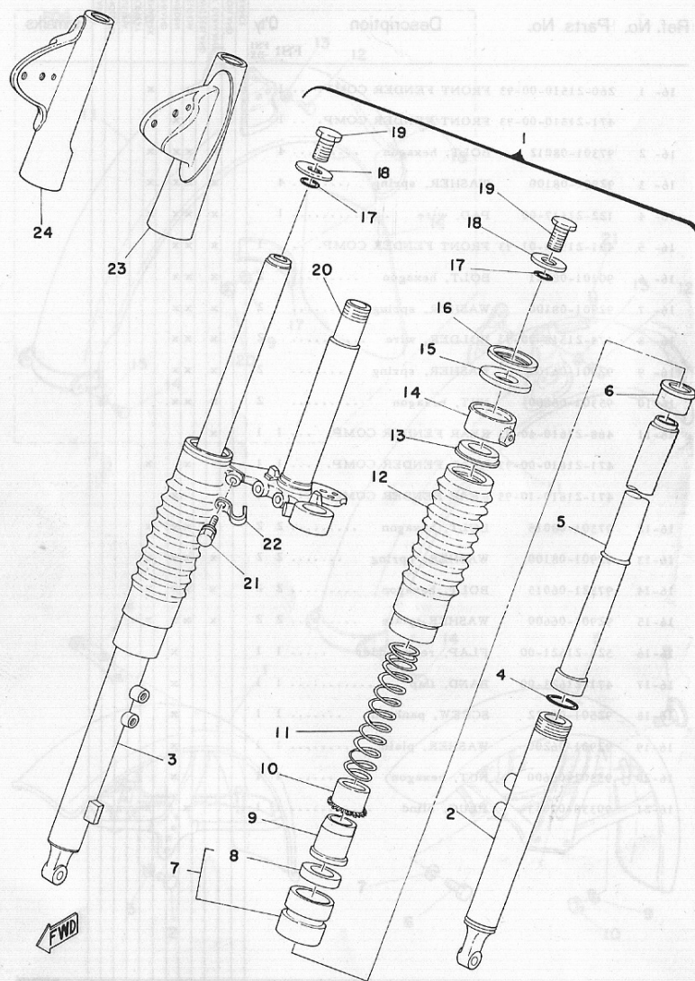
Fig. 17 FRONT FORK
