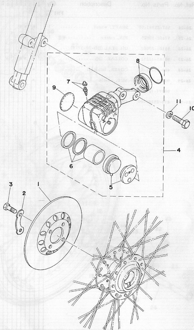
Fig. 27 DISK BRAKE • CALIPER
