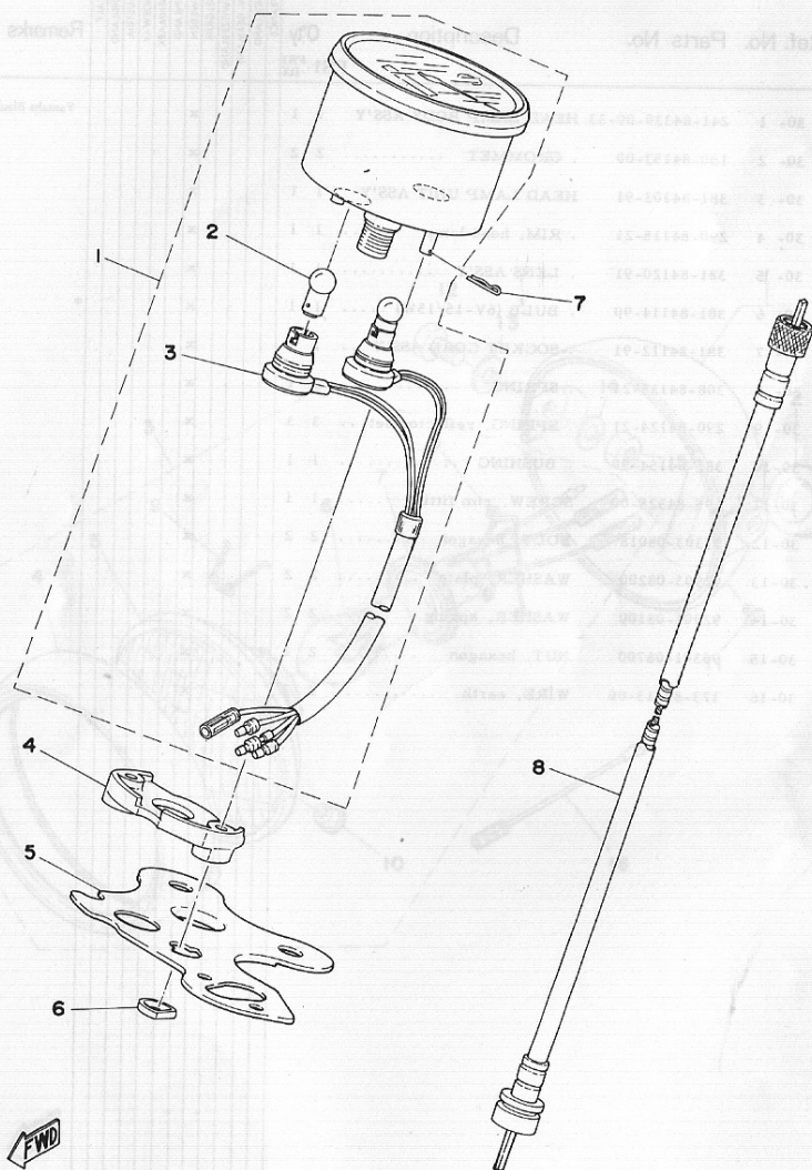
Fig. 31 SPEEDOMETER
