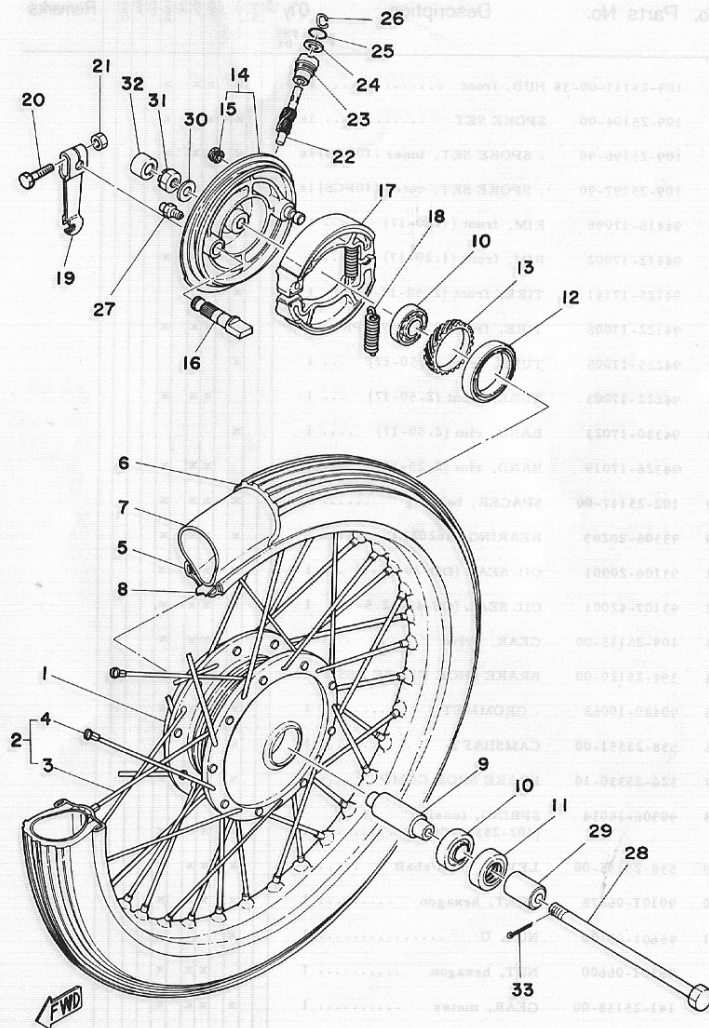
Fig. 25 FRONT WHEEL
