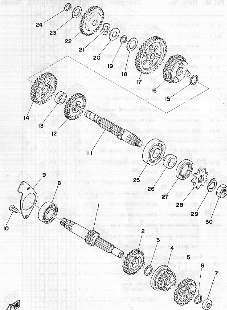
Fig. 5 TRANSMISSION
