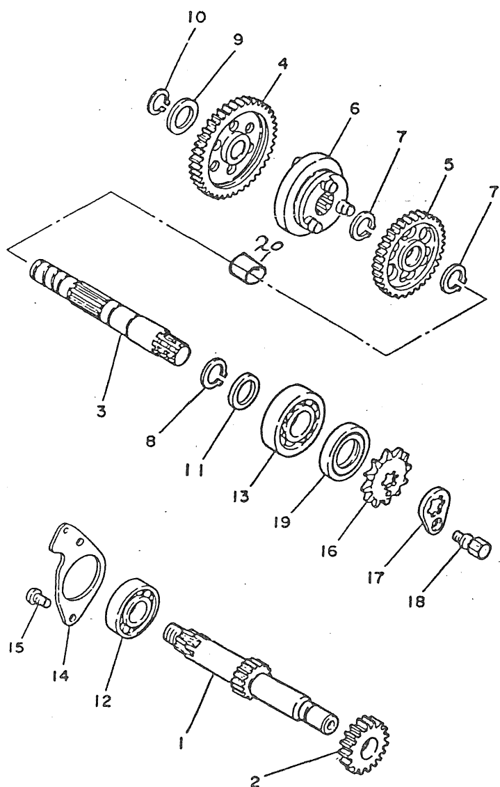
FIG. 10 TRANSMISSION
