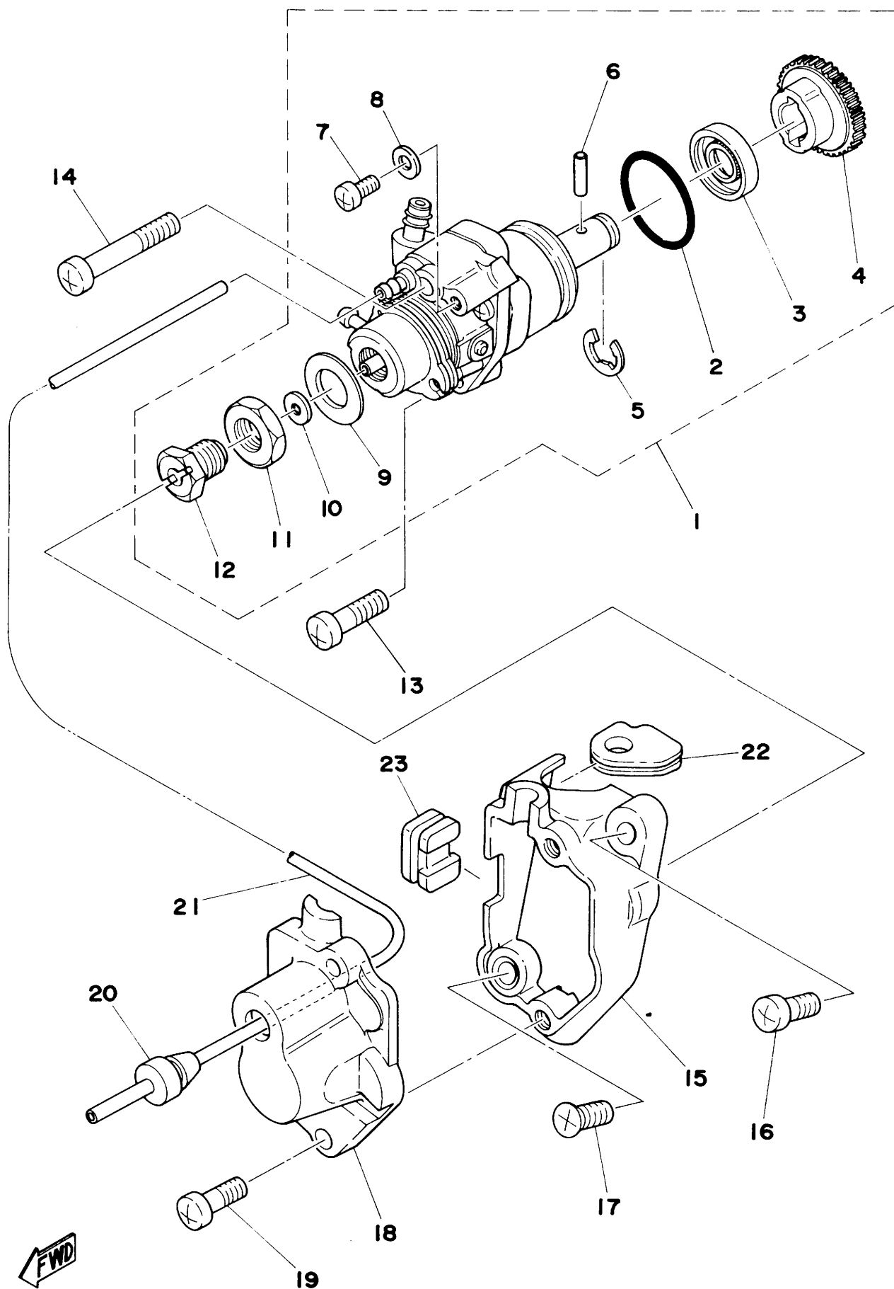
Fig. 11 OIL PUMP
