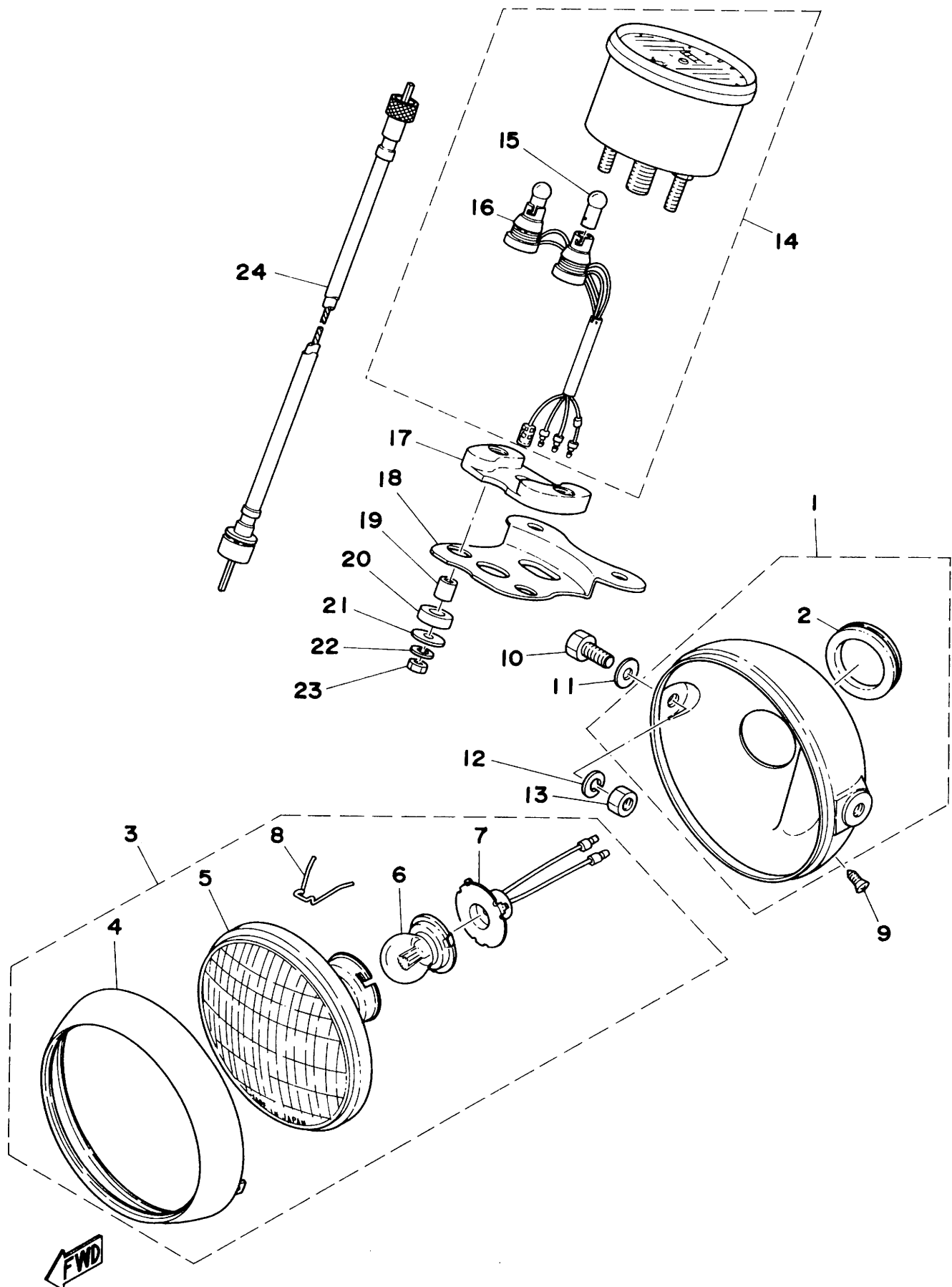
Fig. 25 HEAD LAMP · SPEEDOMETER
