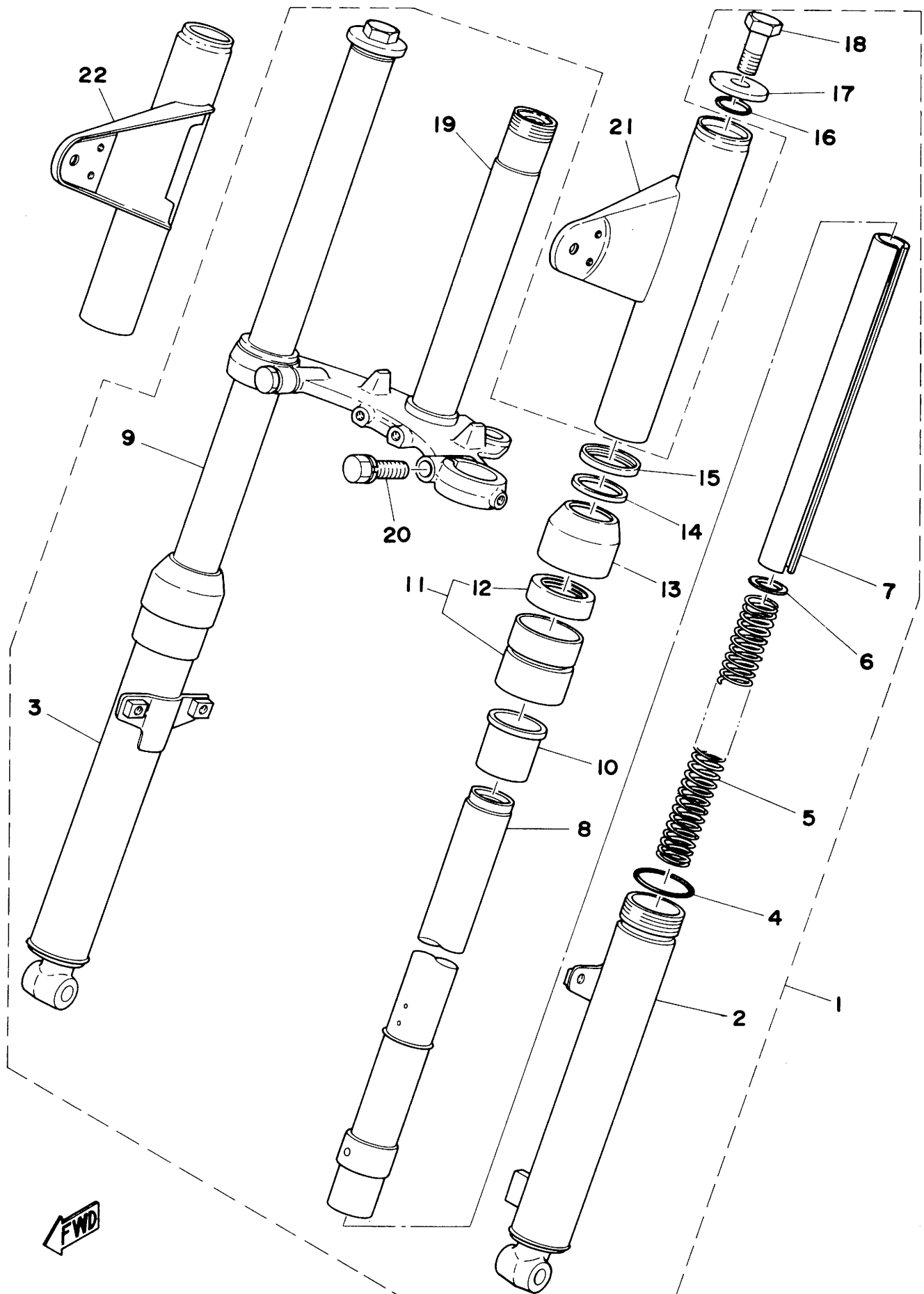
Fig. 17 FRONT FORK
