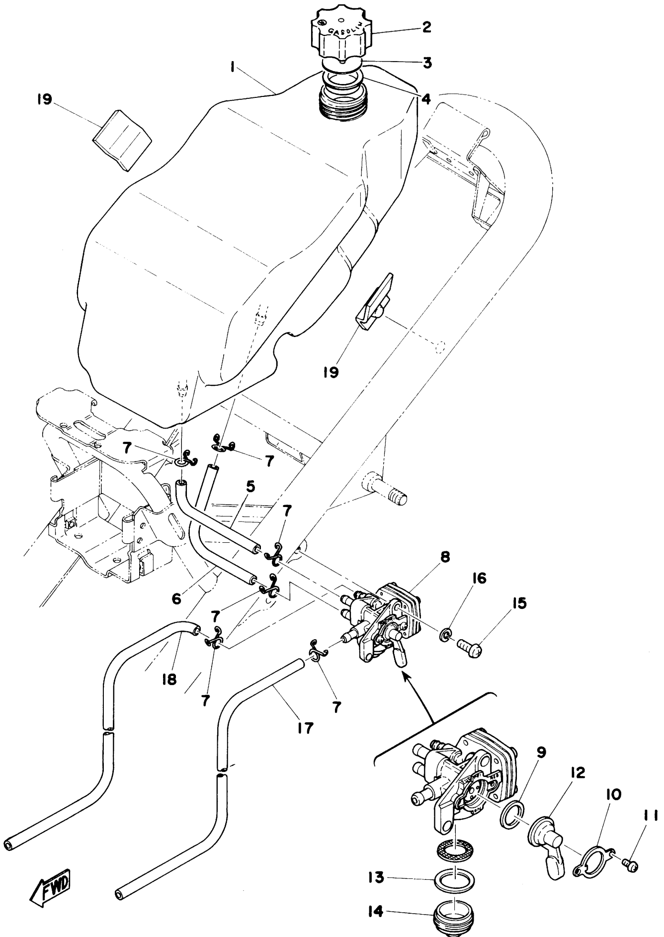
Fig. 20 FUEL TANK
