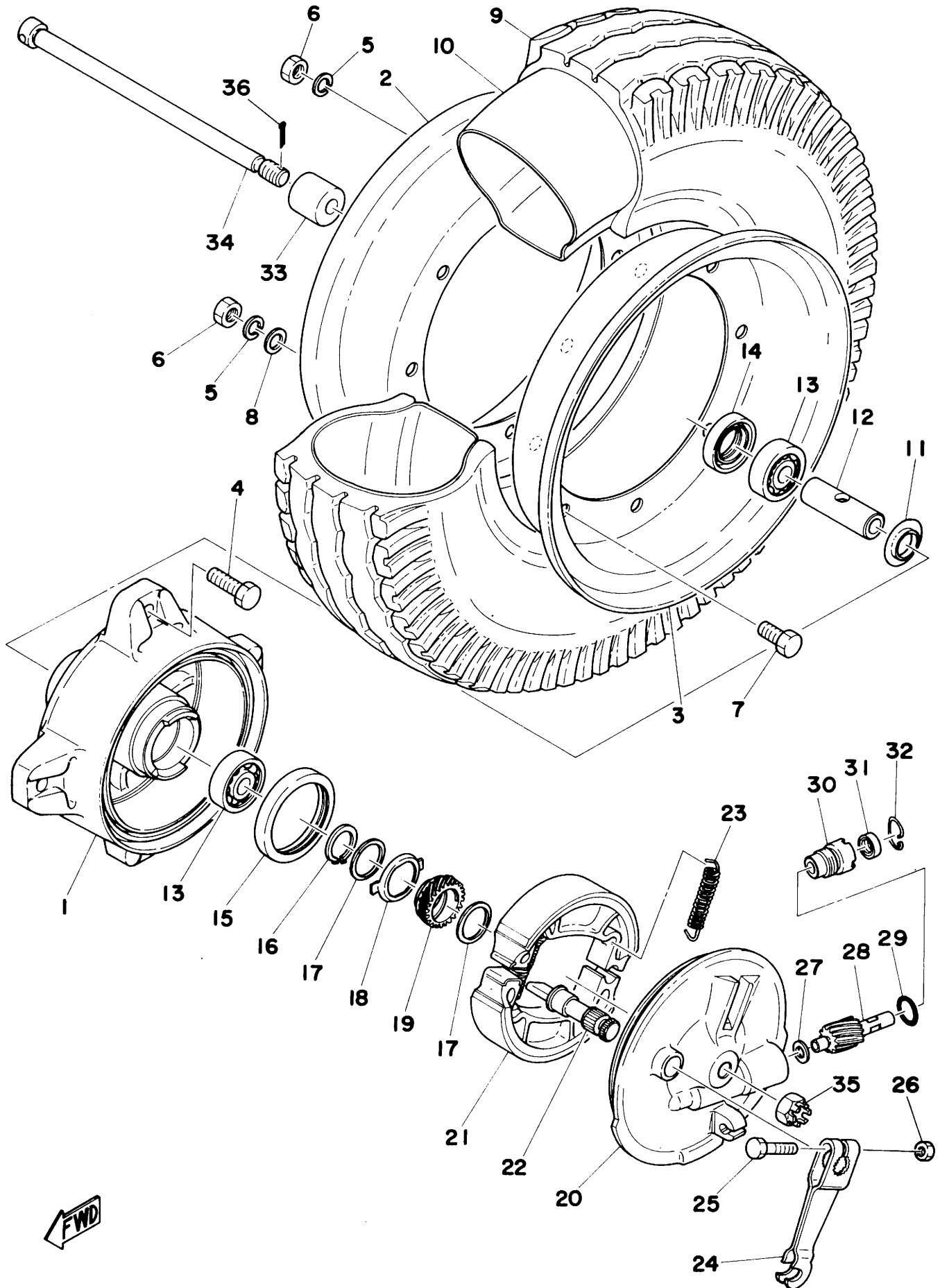
Fig. 23 FRONT WHEEL
