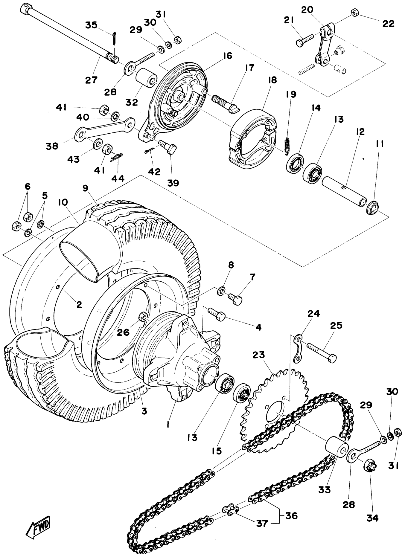
Fig. 24 REAR WHEEL
