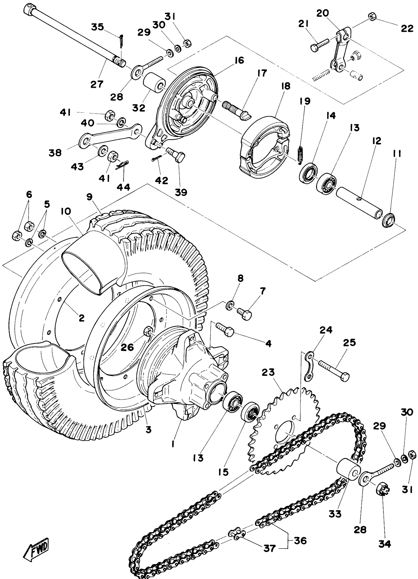
Fig. 24 REAR WHEEL
