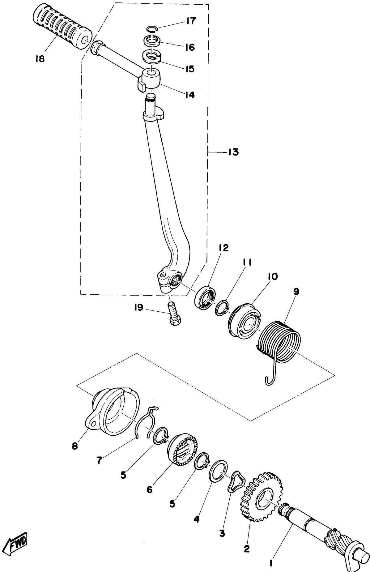
Fig. 7 KICK STARTER
