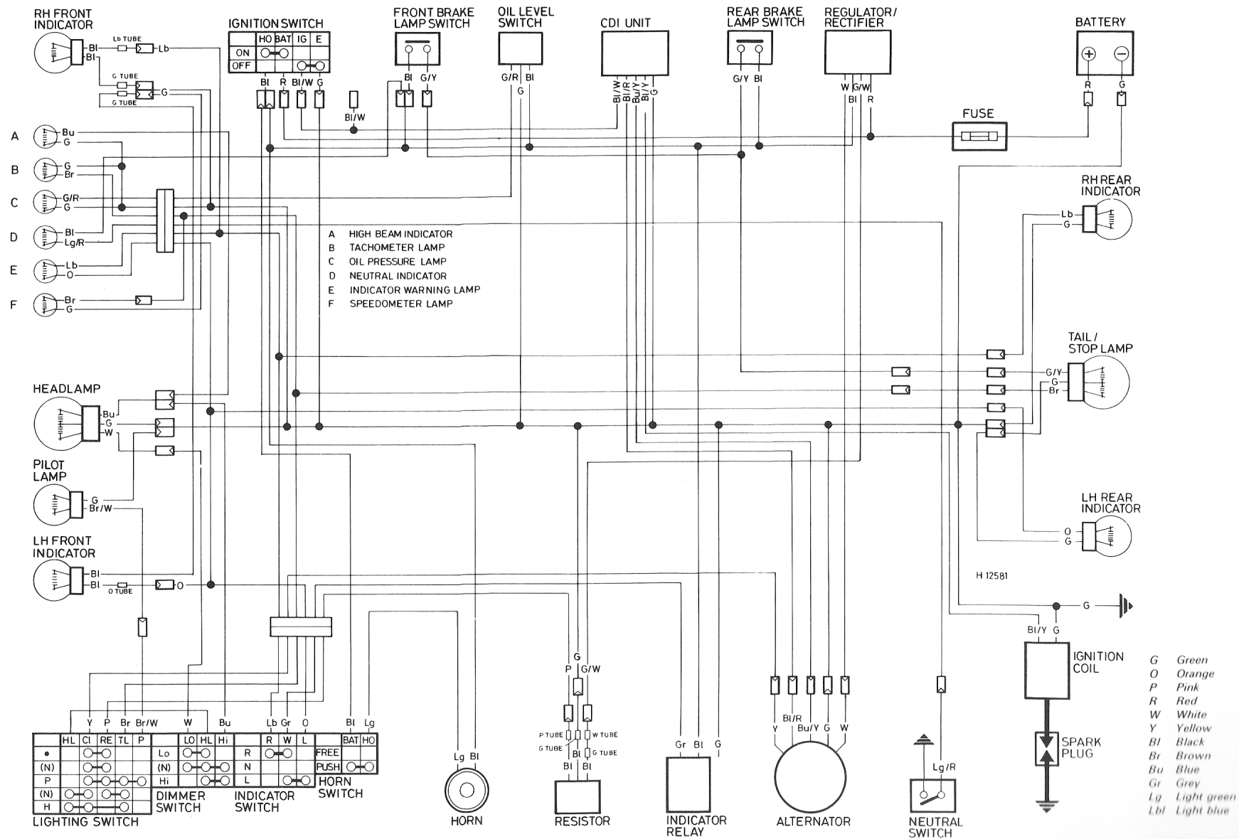
Wiring diagram – MTX50 S-C
