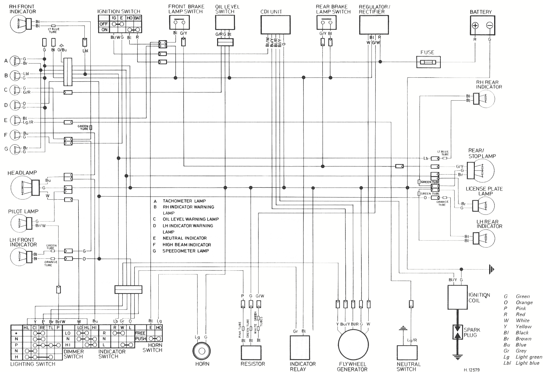
Wiring diagram – MBX50 S-D
